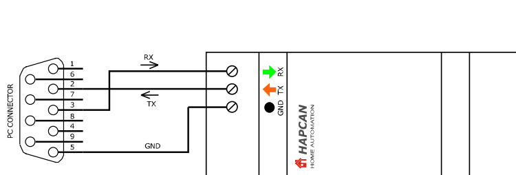
Figure 1. RS232C connector.
